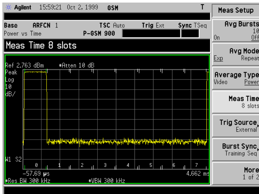
Figure 3-9 Power vs Time Measurement Result - Monitor View
