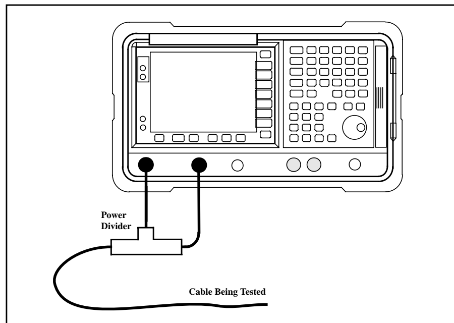
Figure 5-1 Cable Fault Location Measurement Set-up
