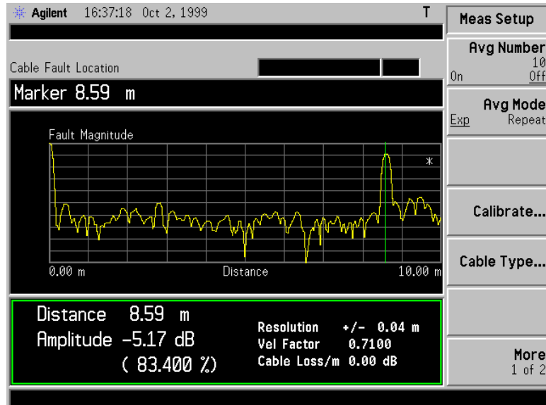
Figure 5-3 Example Cable Fault Location Measurement Screen
