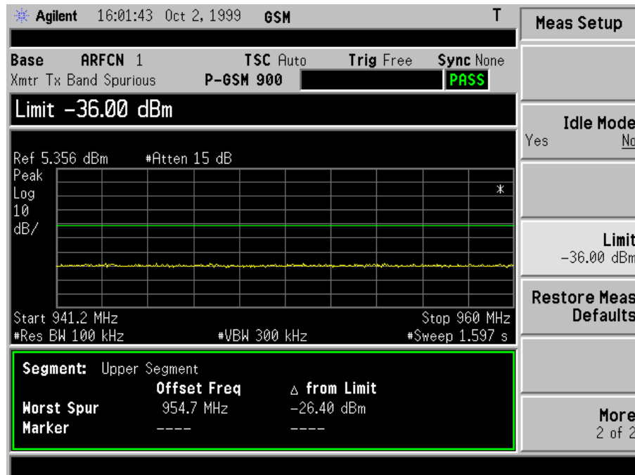
Transmitter Tx Band Spurious Measurement Results
