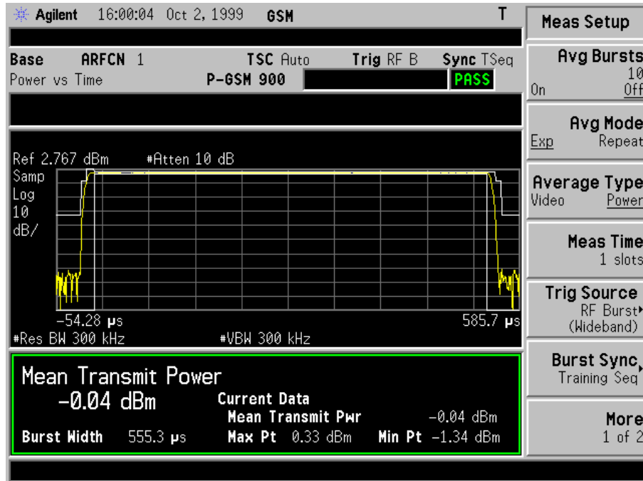
Figure 3-8 Power vs Time Measurement Result - Mask View
