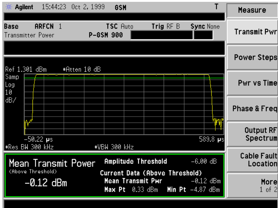
Figure 3-11 Transmitter Power Result - Single Burst
