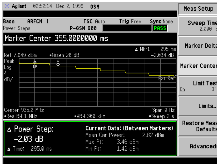
Figure 3-10 Power Steps Measurement
