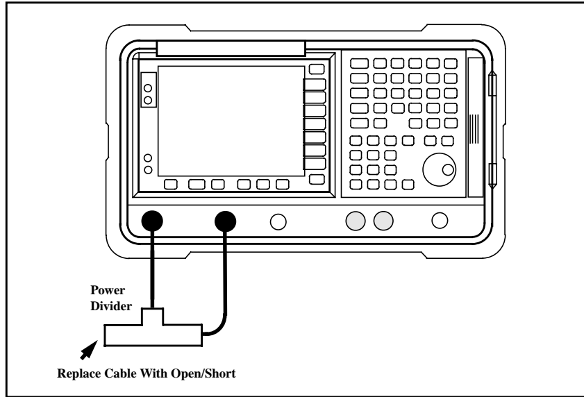
Figure 5-2 Calibrating the spectrum analyzer for cable fault location
