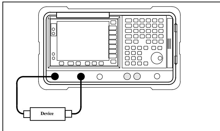
Figure 5-7 Loss/Gain Measurement Set-up
