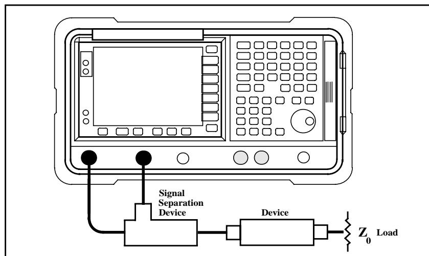
Figure 5-4 Return Loss Measurement Set-up
