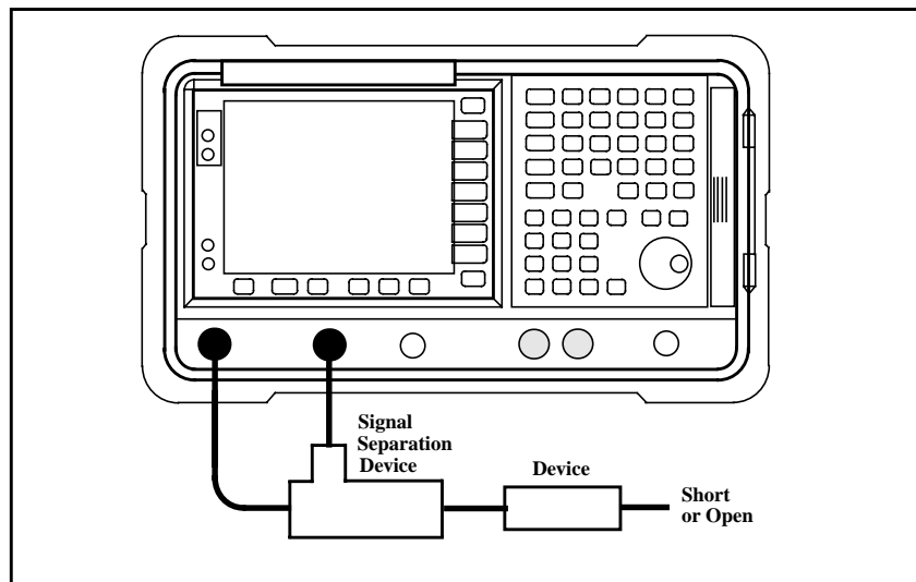
Figure 5-5 Calibrating the Spectrum Analyzer for Return Loss
