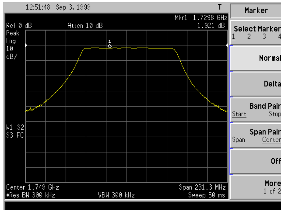
Figure 5-8 Example Loss/Gain Measurement for a Bandpass Filter
