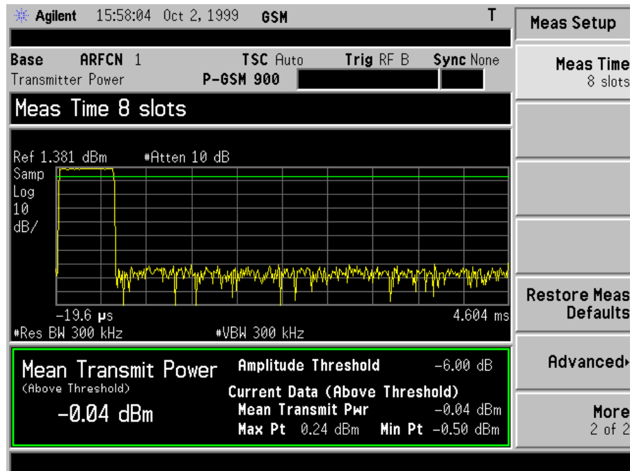
Figure 3-12 Transmitter Power Result - Multiple Bursts
